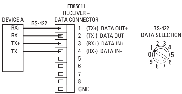
RS-422 DATA CONNECTIONS BETWEEN DEVICE A AND FR85011 RECEIVER
